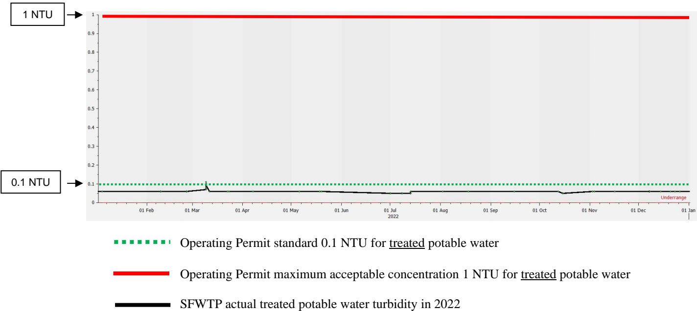
Graph 1 – potable water turbidity at the SFWTP
